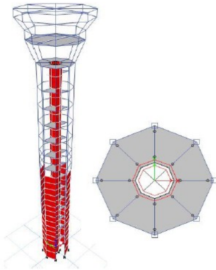
Fig. A Fig. B Fig. 4 Octagonal Elevation and Plan
