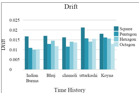
Fig. 7 Story Drift of different shapes of ATCTs
