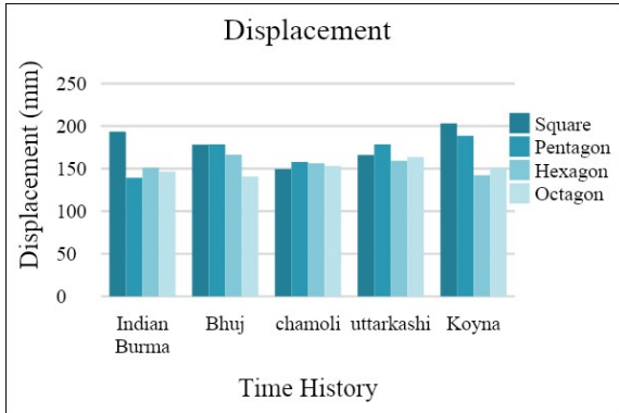
Fig. 6 Story Displacement of different shapes of ATCTs
