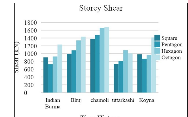
Fig. 8 Story Shear of different shapes of ATCTs
