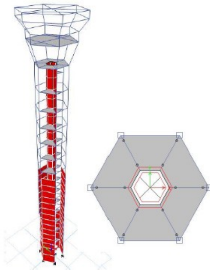
Fig. A Fig. B Fig. 5 Hexagonal Elevation and Plan
