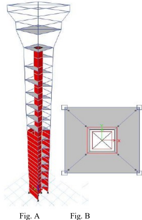
Fig. 2 Square Elevation and Plan
