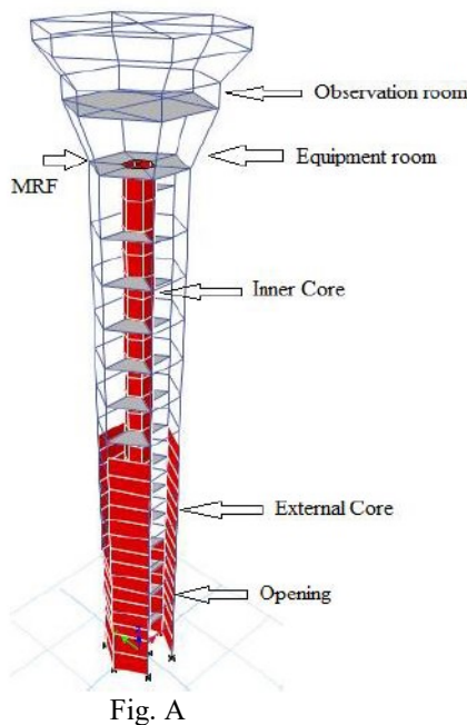
Fig. 1 Elevation of the ATC considered
