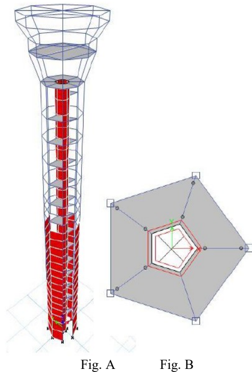
Fig. 3 Pentagonal Elevation and Plan
